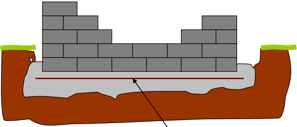
Foundation reinforced with 3/8'' Rebar
